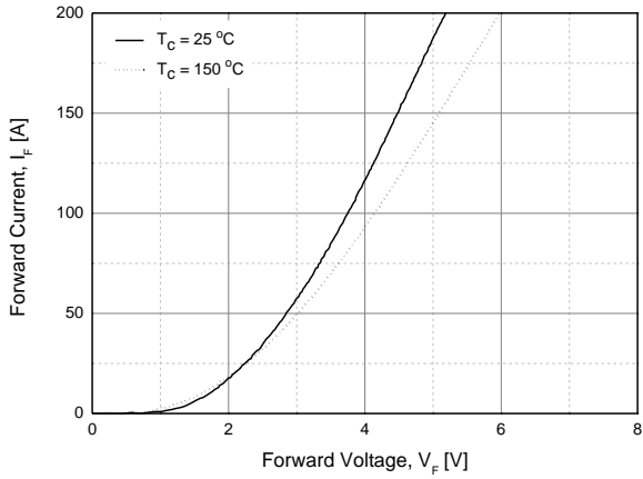
Fig. 18 Conduction characteristics
