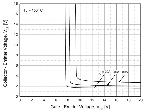
Fig. 5 Saturation voltage vs. gate bias
