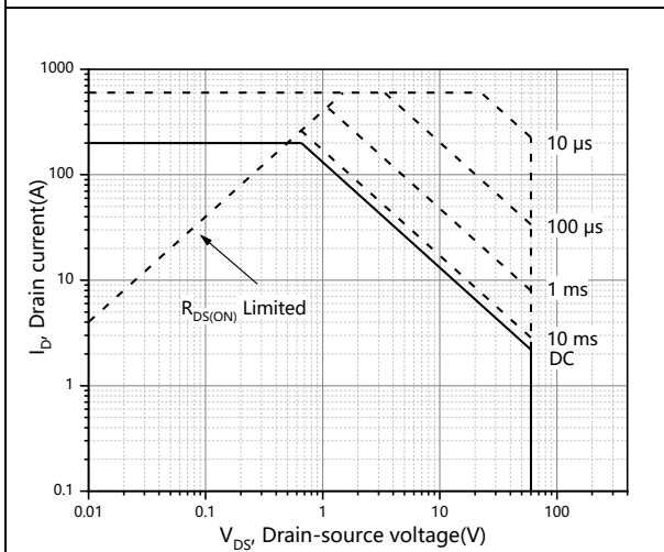
Figure 11. Safe operation area for T C =25 °C
